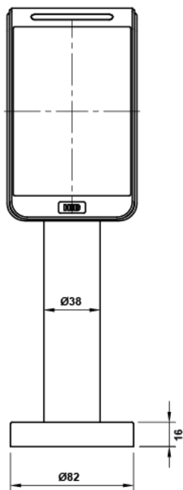
Vista Frontal
